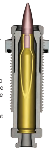
NO CRIMP GROOVE REQUIRED—EVEN WITH JACKETED BULLETS
